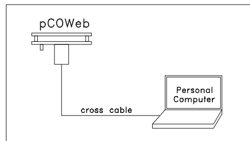
Figure 3.a - Direct PC- pCOWeb connection
